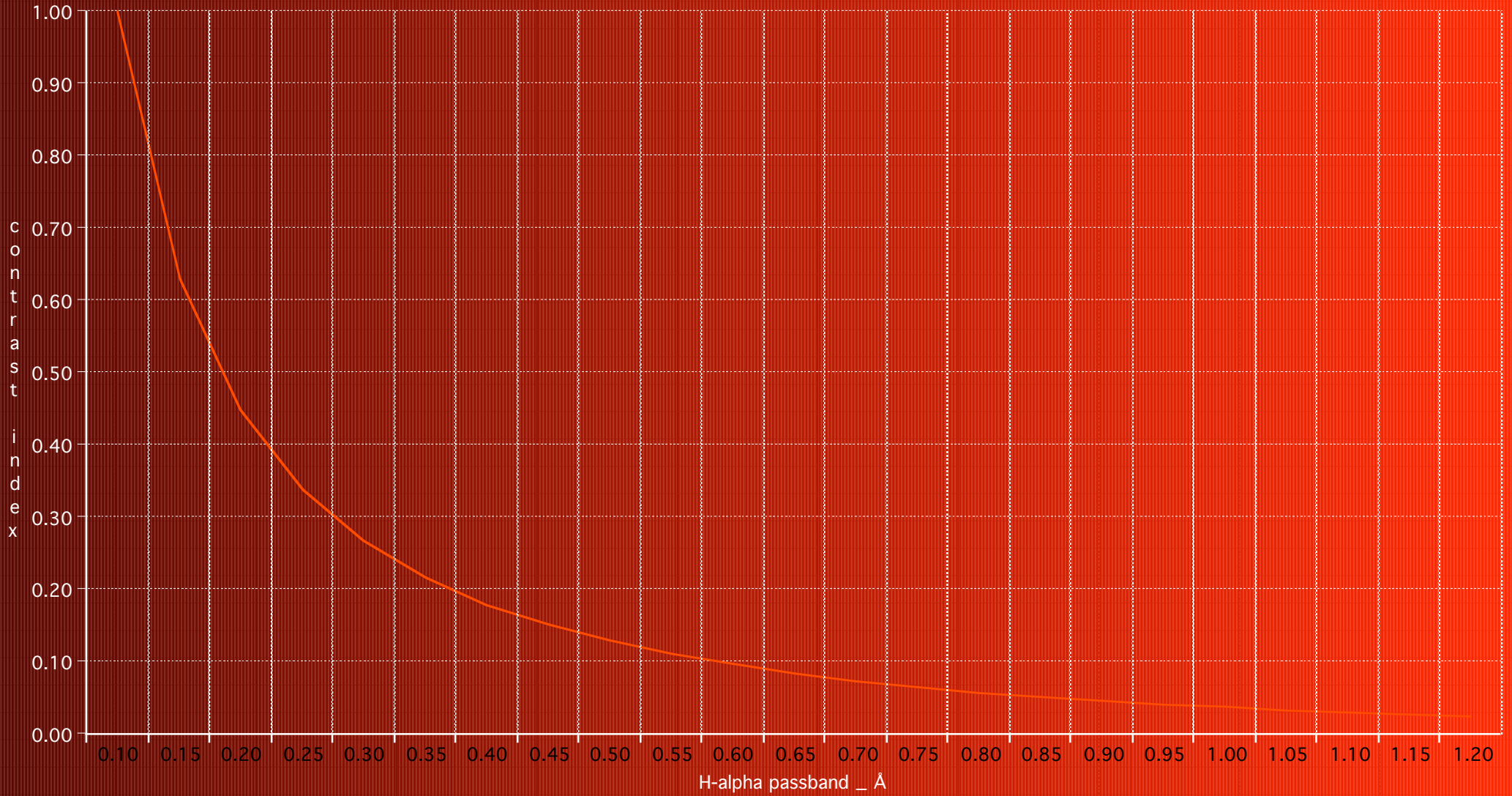
relative image contrast vs H-alpha passband
