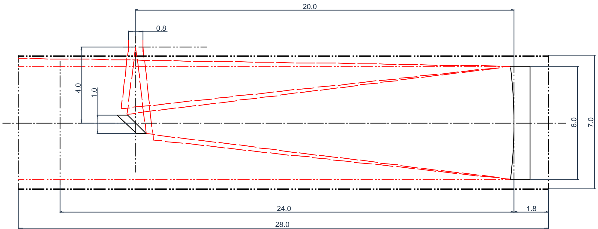
6-inch f/4 RFT with 1-inch minor axis flat
