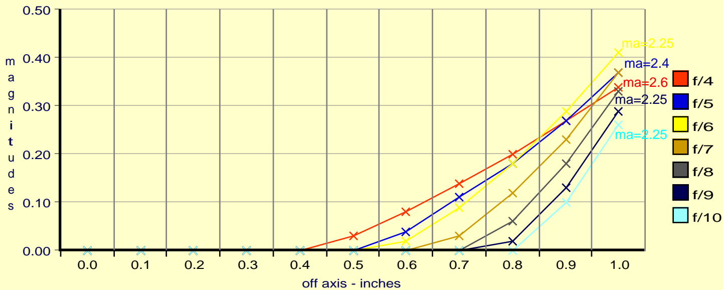
Case 1: vignetting_1/2 degree field of view
