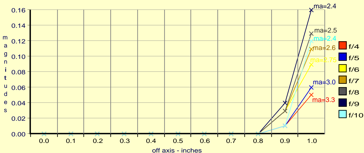
Case 2: vignetting_1-3/4-inch linear field of view
