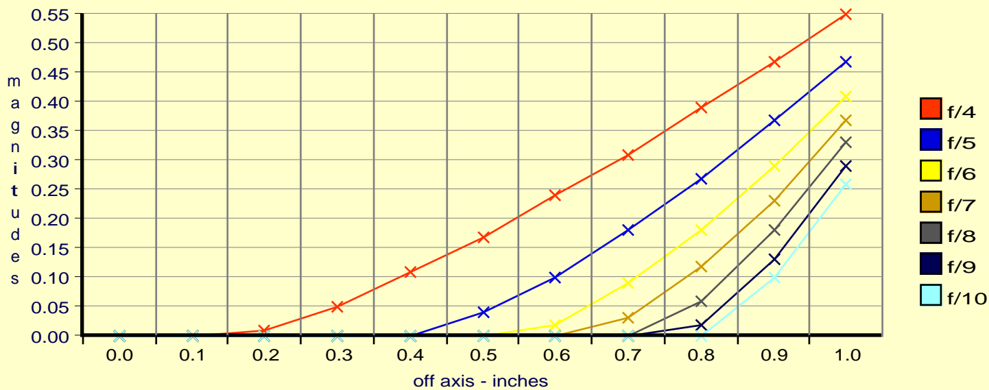
Case 3: vignetting_2-1/4-inch minor axis diagonal
